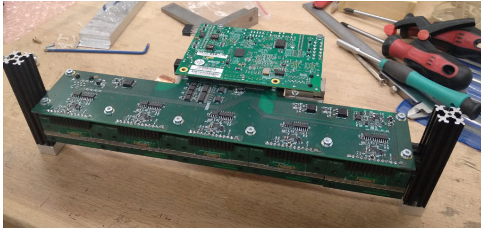
Fig. 2-2 The electronics (both boards connected together, without additional shielding on the FPGA board)
