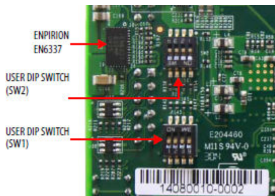
Fig. 2-15 Important DIP-switches
