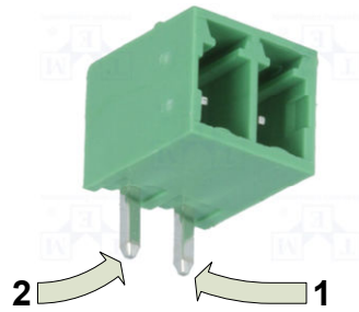
Fig. 2-19 Power connector pin numbering
