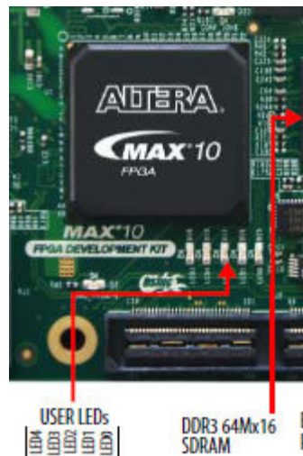
Fig. 2-16 LED placement
