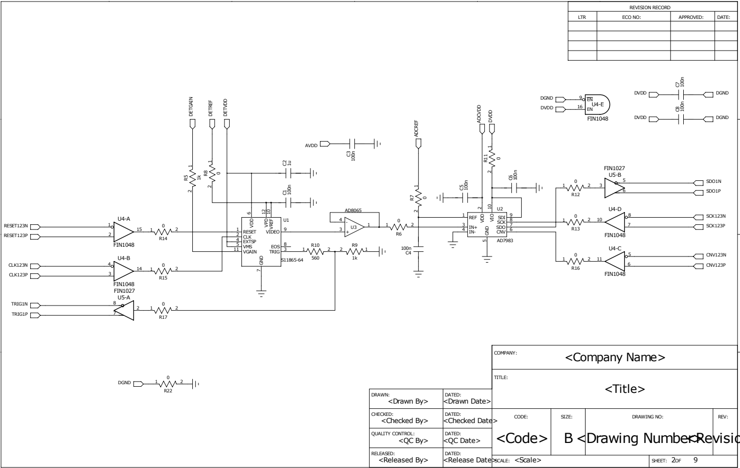
Fig. 2-5 Schematics diagram 2/9
