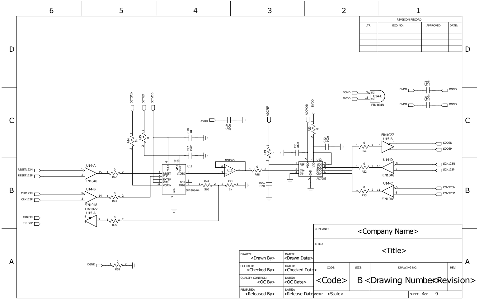
Fig. 2-7 Schematics diagram 4/9
